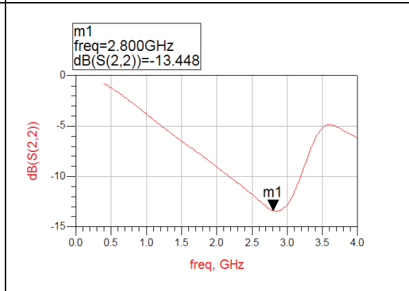
Figure 121. S22 tuned for 2.8GHz
