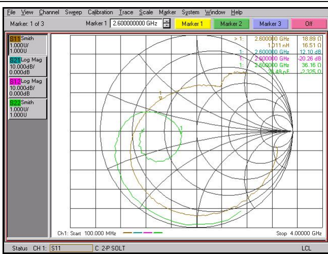
Figure 82. S11 and S22, Smith Chart
