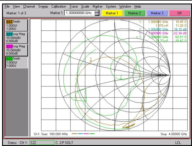
Figure 58. S11 and S22, Smith Chart
